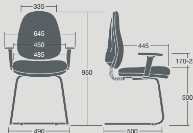
TEPC/1D: Overall Dimensions: 645w x 600d x 950h
