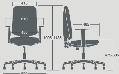
EDE/FA: Overall Dimensions: 690w x 690d x 1185h
