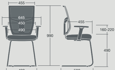
TPMC/1D: Overall Dimensions: 645w x 575d x 990h
