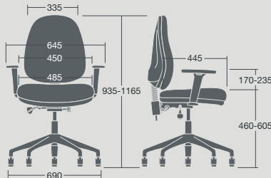
TEP/1D: Overall Dimensions: 690w x 690d x 1165h
