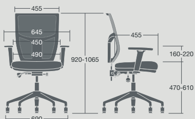
TPM/1D: Overall Dimensions: 690w x 690d x 1065h
